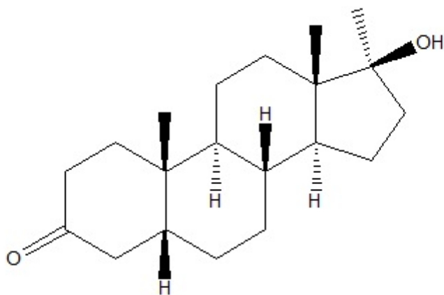
17a-methyl-17b-hydroxy-5b-androstan-3-one
