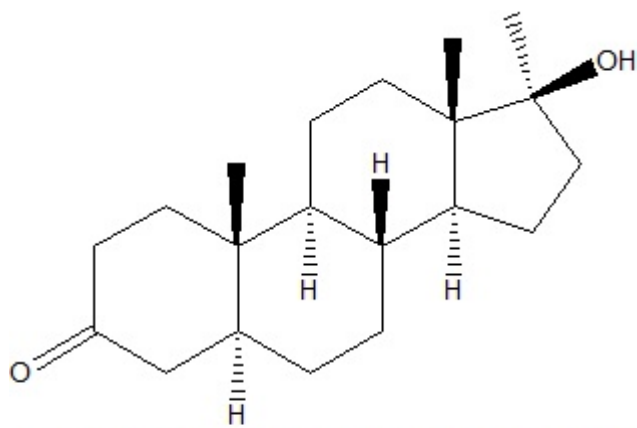
17a-methyl-17b-hydroxy-5a-androstan-3-one
